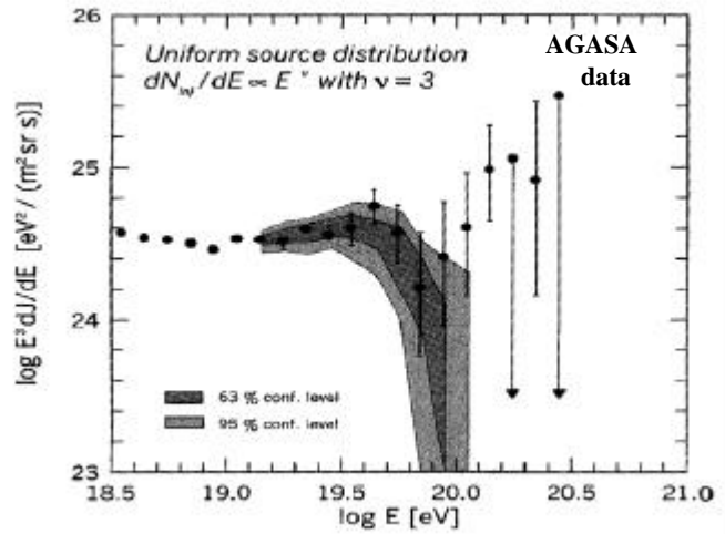
Fig. 1.1 – Energy spectrum and GZK cutoff
