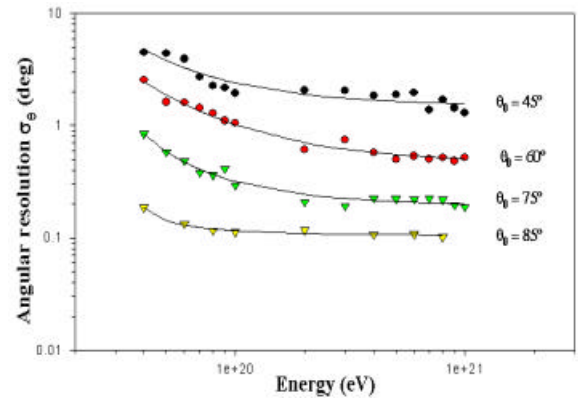
Fig.1.5 - Angular resolution of showers (see text) [33].
